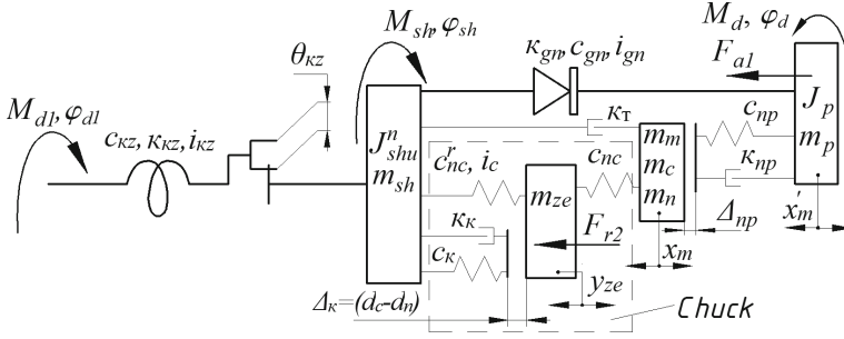
Fig. 1. The dynamic model of the new ACM [3] as a part of CM of the lathe.
