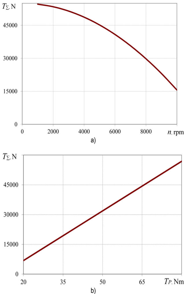
Fig. 4. Dependence of clamping force T_{\Sigma} in proposed CM from: a) frequency of rotation of the spindle n when the torque of the rotor of T_p = 66 \text{ Nm} ; b) torque T_p , which appears on the rotor at frequency of the spindle rotation n = 5000 \text{ rpm}
