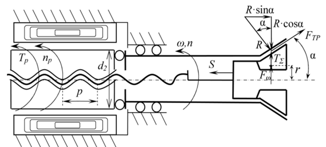
Fig. 3. The scheme for calculating CM parameters
