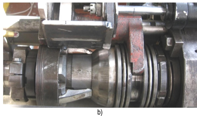
Fig. 1. Mechanical CM's actuator with geometric locking: a) functioning scheme in combination with a lever chuck (in the "clamped" state); b) general view of the mechanism (in the "unlocked" state)
