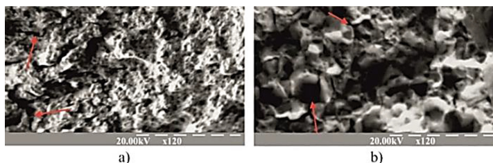
Fig. 3. Fractogram of alloy HX – Alloy Type 66Ni-17Cr after heat treatment at 900 °C ( \times 120 ): a) near the cut; b) in the sample center.
