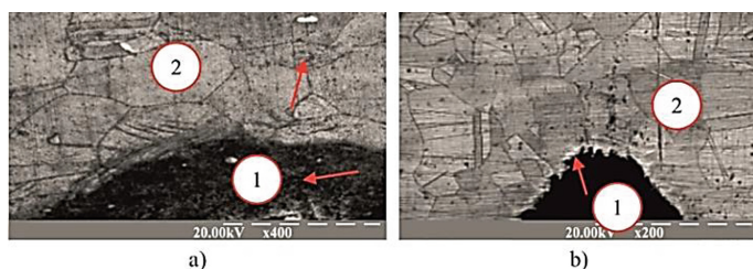
Fig. 4. The structure of the etched surface layer of the alloy HX – Alloy Type 66Ni-17Cr (1 – subsurface layer, 2 – base metal): a) before exploitation ( \times 400 ); b) after exploitation ( \times 200 ).
