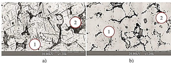
Fig. 5. \sigma -phase in the alloy HX – Alloy Type 66Ni-17Cr ( \times 1200 ); (1 – plates of the \sigma -phase in the main matrix; 2 – the base metal): a) after exploitation; b) after dissolution as a result of additional heat treatment.
