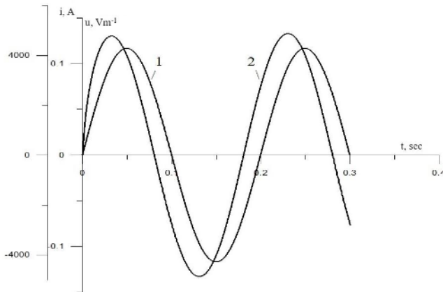
Fig. 3. Calculated curves of current (1) and voltage per unit length (2) of the slot current conductor in the state of sudden switching on the current source I = 4282 \sin(31.4t) . Groove dimensions: h \times l \times a = 0.038 \text{ m} \times 0.23 \text{ m} \times 0.005 \text{ m}
